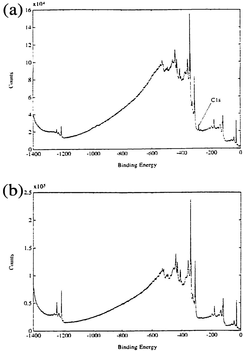
Figure 1.9. XPS spectra from a Ge sample. a) As-etched surface, and b) Clean surface after cycles of ion milling and thermal annealing.
