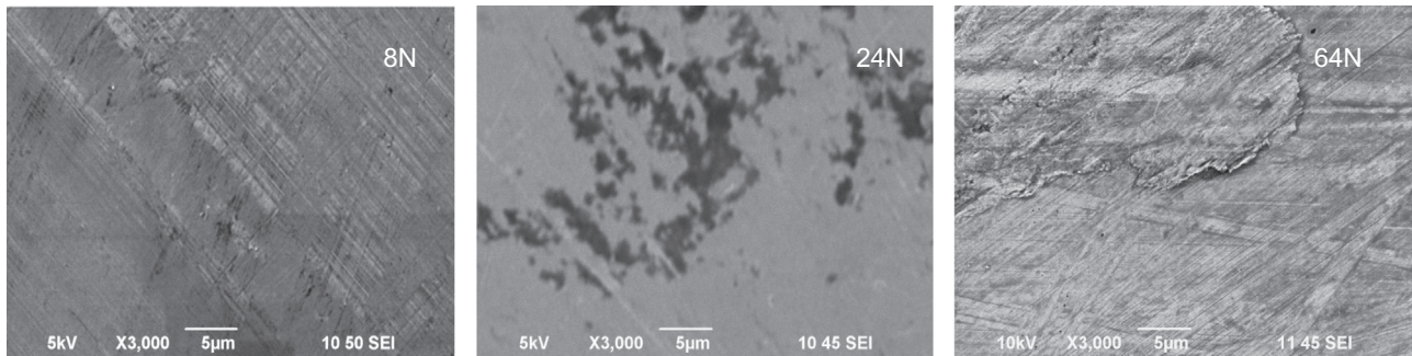
Fig. 7. SEM analysis. The 8 N samples showed only slight scratching on the surfaces. Higher load levels caused the appearance of tribofilms, as shown exemplified for a 24 N sample. The samples of the highest load category were most damaged.
