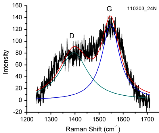
Fig. 8. Raman spectrum of tribofilm on a 24 N sample. The D (cyan) and G (blue) lines of graphitic carbon are shown. The tribofilm signal is fitted by two Gaussian peaks (red). (For interpretation of the references to color in this figure legend, the reader is referred to the web version of this article.)
