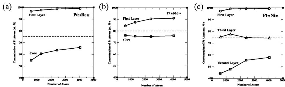
Fig. 5 (a)–(c) The calculated Pt fraction on the surface layer and in the core region as a function of size in (a) Pt 3 Re and (b) Pt 4 Mo particles at 600 K. The dashed line shows the overall Pt concentration in the particle. (c) The calculated Pt fraction in the first three layers as a function of size in Pt 3 Ni particles at 600 K. The dashed line shows the overall Pt concentration in the particle. Reproduced with permission from ref. 80.
