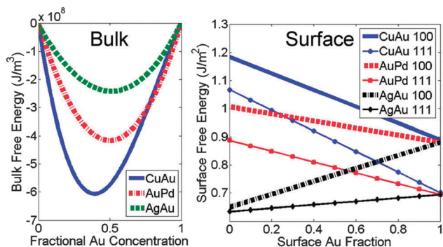
Fig. 2 Fitted bulk and surface free energy for CuAu, AuPd, and AgAu. The bulk free energy is defined as the deviation from the linear interpolation between two pure elements. The surface free energy is assumed to vary linearly between two pure surfaces.
