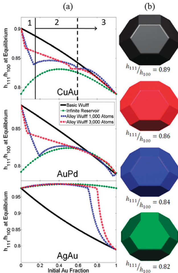
Fig. 4 Shape dependence on size and homogeneous composition of the particles, parameterized by (h_{111}/h_{100}) . (a) Shape as a function of homogeneous composition of Au for 'basic Wulff' model (black), 'infinite reservoir approximation' (green) and alloy Wulff model for two particle sizes (blue for 1000 atoms, red for 3000 atoms). (b) Shape variations of CuAu alloy particles with a homogeneous Au concentration of 0.15, according to respective models.
