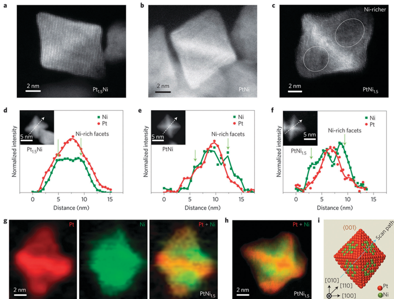
Fig. 9 Atomic-resolution Z-contrast images, EELS linescans and mappings of \text{Pt}_x\text{Ni}_{1-x} octahedral nanoparticles. (a)–(c) Z-contrast images of octahedral particles close to \langle 110 \rangle zone axis of (a) \text{Pt}_{1.5}\text{Ni} , (b) \text{PtNi} , (c) \text{PtNi}_{1.5} . (d)–(f) EELS linescans of octahedral nanoparticles close to \langle 100 \rangle zone axis of (d) \text{Pt}_{1.5}\text{Ni} , (e) \text{PtNi} , (f) \text{PtNi}_{1.5} . The linescans are along the [110] direction, passing through the longest axis. The insets are the Z-contrast images of the corresponding particles. (g) EELS elemental map of \text{PtNi}_{1.5} octahedral nanoparticle showing preferential segregation of Ni (green) to the \langle 111 \rangle facets, and Pt (red) enriched edges and corners. (h) A composite image of a HAADF image showing Pt red, and an EELS elemental map showing Ni green. (i) Ball schematic showing the octahedral particle along the \langle 001 \rangle zone axis, with Ni-rich facets and Pt-rich frame. Reproduced with permission from Macmillan Publishers Ltd: Nature Materials ref. 35, copyright 2013.
