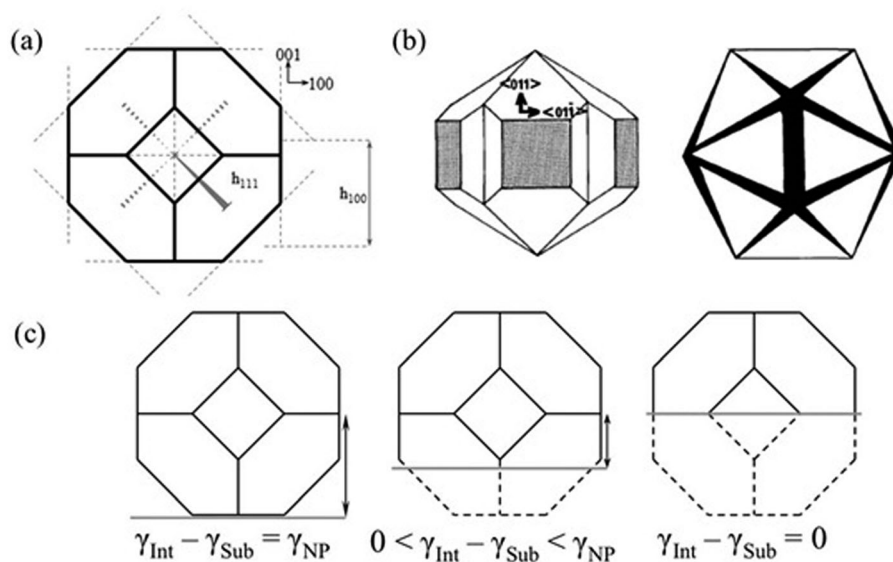
Fig. 1 (a) Conventional Wulff construction, (b) modified Wulff construction, with twin boundaries introduced, (c) Winterbottom construction, with substrate effects included.
