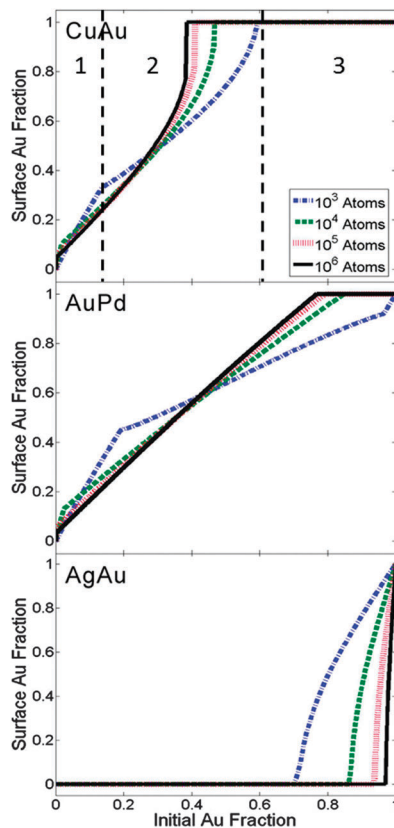
Fig. 3 Effect of size and initial composition on the equilibrium surface composition of alloy particle. Curves for 10^3 , 10^4 , 10^5 and 10^6 atoms ( \sim 3 , 7, 15 and 30 nm in diameter) are plotted as a function of overall composition. The three regimes can be observed in CuAu and AuPd particles, while only two regimes can be seen for AgAu.
