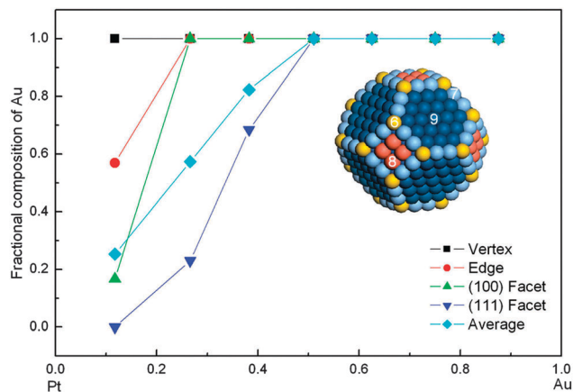
Fig. 6 Composition fraction of Au at different sites (vertex and edge) and facets ((100) and (111)) as a function of overall Au composition for particles containing 586 atoms. Reproduced with permission from ref. 76. Copyright 2010 American Chemical Society.
