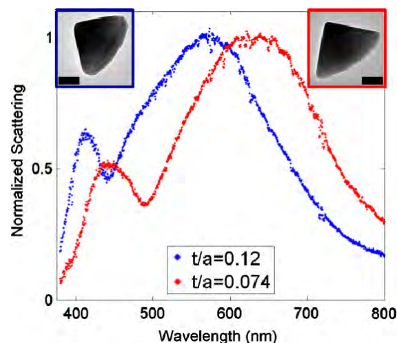
Figure 2. Effect of equatorial corner rounding on the LSPR spectrum of a bipyramid. Blue curve, left inset: round particle ( t/a = 0.12 ). Red curve, right inset: sharp particle ( t/a = 0.074 ). The scale bars are 50 nm.
