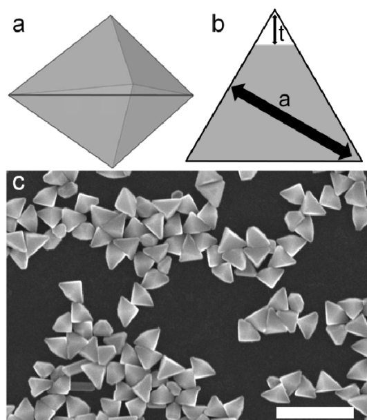
Figure 1. Particle geometry and definition of structural parameters. (a) 3D model of a right bipyramid, (b) structural parameters: truncation length ( t ) and height of the equilateral base ( a ) (c) micrograph of a typical reaction mixture obtained on a Hitachi S4800-II scanning electron microscope. The scale bar in (c) is 500 nm.
