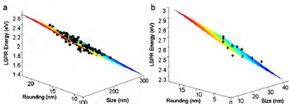
Figure 4. Effect of size and corner rounding on the longitudinal dipolar resonances of nanoparticles. (a) Experimental data on Ag bipyramids (fit described by equation (2)), (b) Ag nanorods based on calculations from Prescott and Mulvaney [57] (fit described by equation S5 available at stacks.iop.org/Nano/23/444005/mmedia ).
