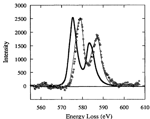
FIG. 9. Cr_{L2,3} EELS spectra from Hg_{1-x}Cr_xSr_2CuO_{4+\delta} (data) are compared with those from CrO_3 and Cr_2O_3 (narrow and bold solid lines, respectively). The absorption energy onset, near-edge structure, and L2/L3 ratios provide a consistent picture that Cr is in a 6+ valence state (as for Cr^{6+} in CrO_3 ).
