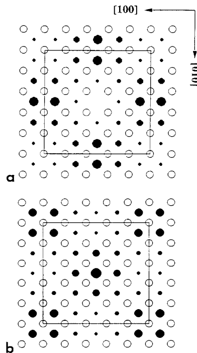
FIG. 6. Average occupancy of Cr atoms at Hg sites for two alternating Hg-O planes along the \langle 001 \rangle axis. The occupancies in (a) and (b) are determined by Eqs. (1) and (2), respectively. Large open circles represent O atoms; solid circles of varying size represent Cr atoms. The sizes of the solid circles are proportional to the Cr fractional occupancies. The Hg occupancy is one minus the Cr occupancy.
