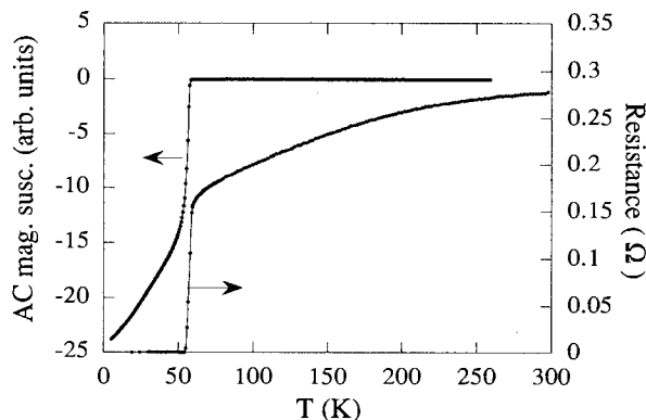
FIG. 1. Resistivity and ac magnetic susceptibility measurements for (\text{Hg}_{1-x}\text{Cr}_x)\text{Sr}_2\text{CuO}_{4+\delta} showing a sharp superconducting transition around 60 K.
