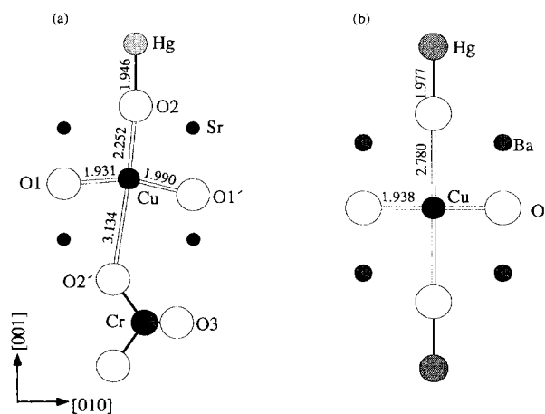
FIG. 3. (a) Proposed local structure for \text{Hg}_{1-x}\text{Cr}_x\text{Sr}_2\text{CuO}_{4+\delta} based on refinement of an average structure model of the fundamental cell dimensions using neutron-powder-diffraction data. Cr atoms achieve tetrahedral coordination by displacing the apical oxygen atoms to a new site [\text{O}(2)'] and incorporating two additional oxygen atoms per Cr atom at the in-plane site \text{O}(3) . The coordinated tilting of \text{CuO}_6 octahedra and spatial constraints on the placement of \text{O}(3) atoms tends to produce the local Cr ordering shown. Bond lengths are in \text{\AA} units. (b) The ideal structure of \text{HgBa}_2\text{CuO}_{4+\delta} (Ref. 14) is shown, for comparison.
