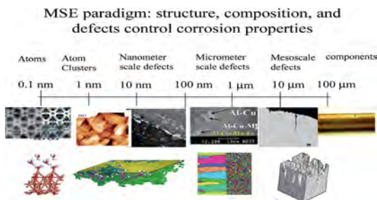
Fig. 2 Hierarchy of the multi-scale corrosion problem starting at the atomic scale and transitioning to the micrometre scale and above. Critical processes at different length scales may factor in to regulate engineering scale corrosion of the copper pipe observed at the far right. It is also noted that the various model length scales from first principles, Monte Carlo, and continuum scale may or may not match the physical or microstructural scale. (Adapted from ref. 60.)
